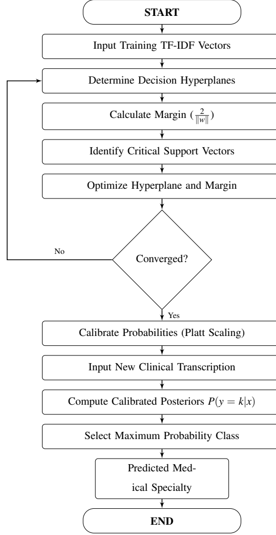
Figure 7: Activity Diagram of Support Vector Machine Classifier
