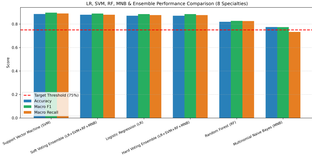
Figure 15: Model Performance Comparison across Accuracy, Macro F1, and Macro Recall against the 75% Target Threshold
