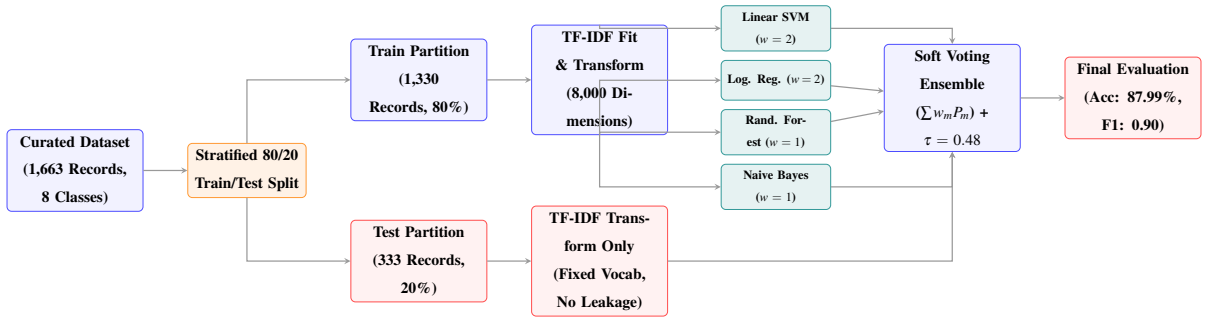
Figure 14: System Design Training, Validation, and Partitioning Workflow
